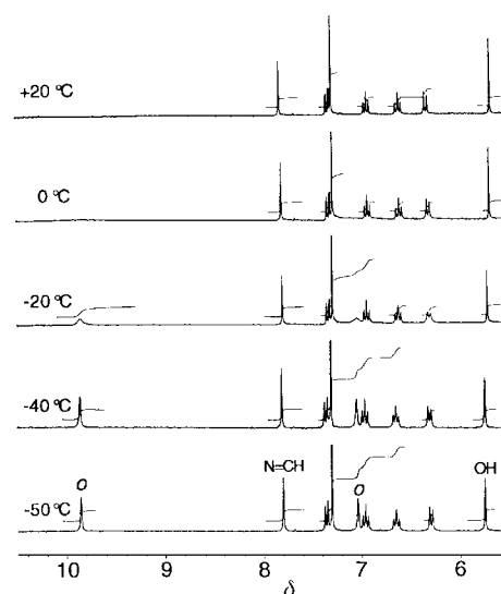
Fig. 2 Variable-temperature 1 H NMR spectra of complex 1 in CDCl 3 from +20 to –50 °C ( o = ortho protons of pendant arm).
